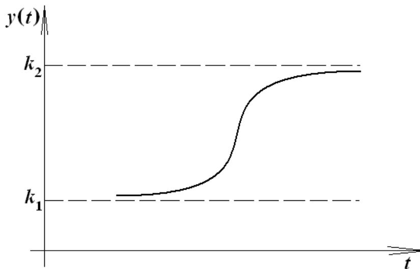
Fig. 1.1. Logistic (S-shaped) curve
